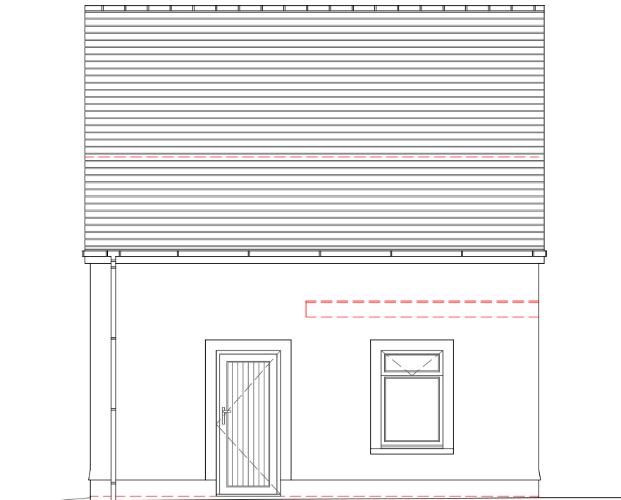
North Elevation
